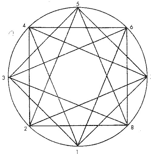
FIGURE 2.0. The 1-skeleton of C(8, 4)
