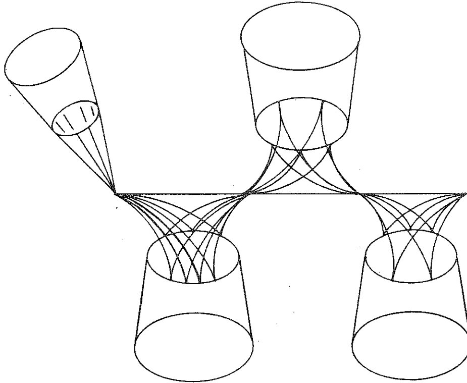
FIGURE 3.3. The complex T_4
