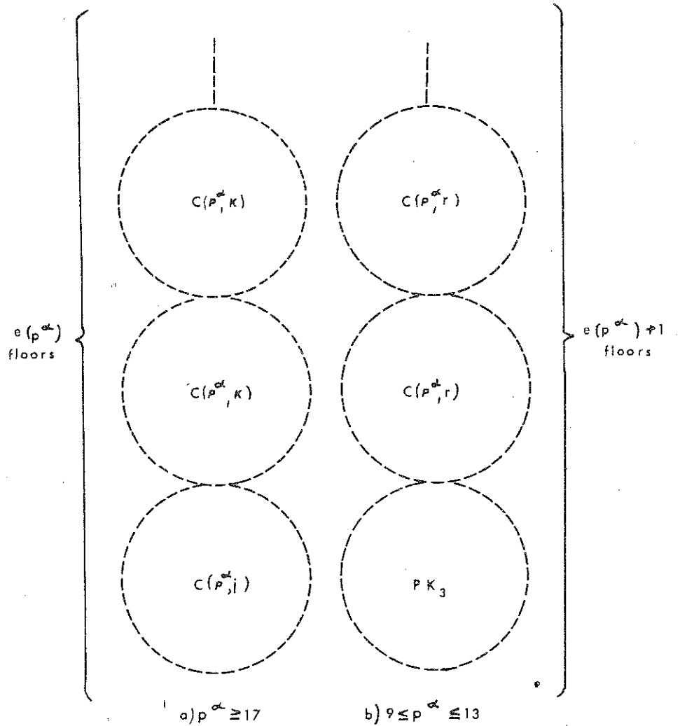
FIGURE 3.5. The complex K^{(n)}(\mathbb{Z}_p^{e(p^\alpha)}) for p^\alpha \geq 9 and n \geq 4
