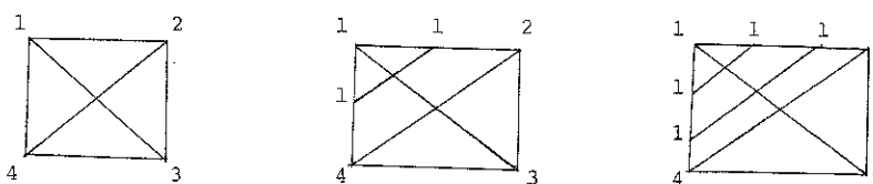
(a) The graphs G^3(4) , G_1(4) , G_2(4)
