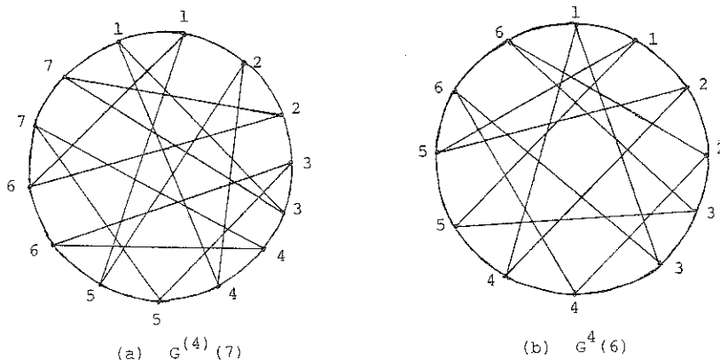
Fig. 5. The graphs G^4(7) and G^4(6) .
