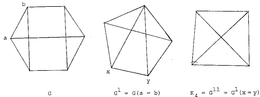
Fig. 1. A composition of two elementary contractions that yields the contraction G \rightarrow K_4 .
