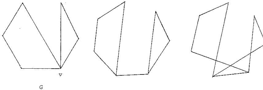
Fig. 2. Two different splittings of G at v .
