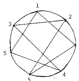
(b) A quartic graph of order 7 and contractibility number 5.
