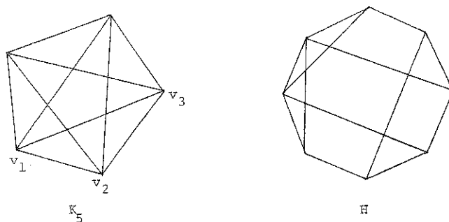
Fig. 3. A graph H \in S^3(K_5; v_1, v_2, v_3) .
